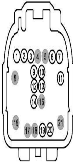
MALE Harness 14334
