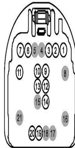
FEMALE Harness 14401
